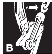
The body cam centre begins to rotate independently of the handle at this stage.
