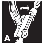
The handle of the BX600 moves freely to the beginning of the release point.
